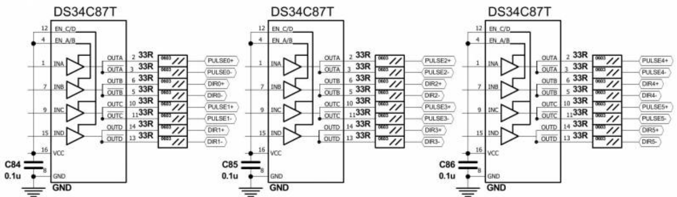
PULSE-DIR channels 0,1,4,5 pinout
